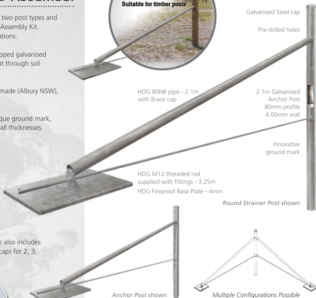
STAY ASSEMBLY Suitable for timber posts
